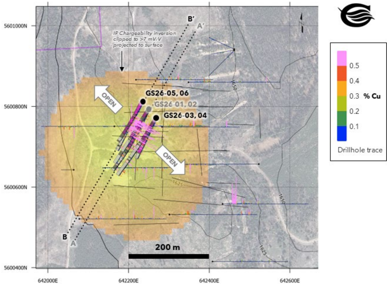
Figure 3: Plan Map of Getty South Drilling.
