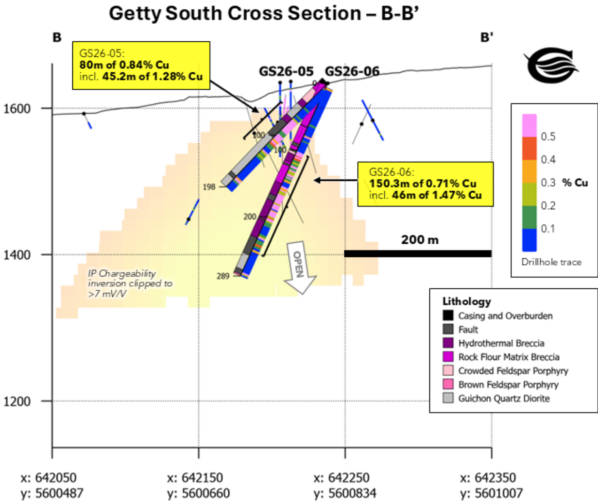
Figure 2: Cross section B-B' through Getty South, showing 2026 and historical drilling and an IP chargeability inversion (50m slice).
